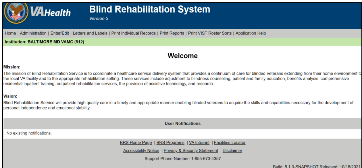
Figure 2: Welcome Page
