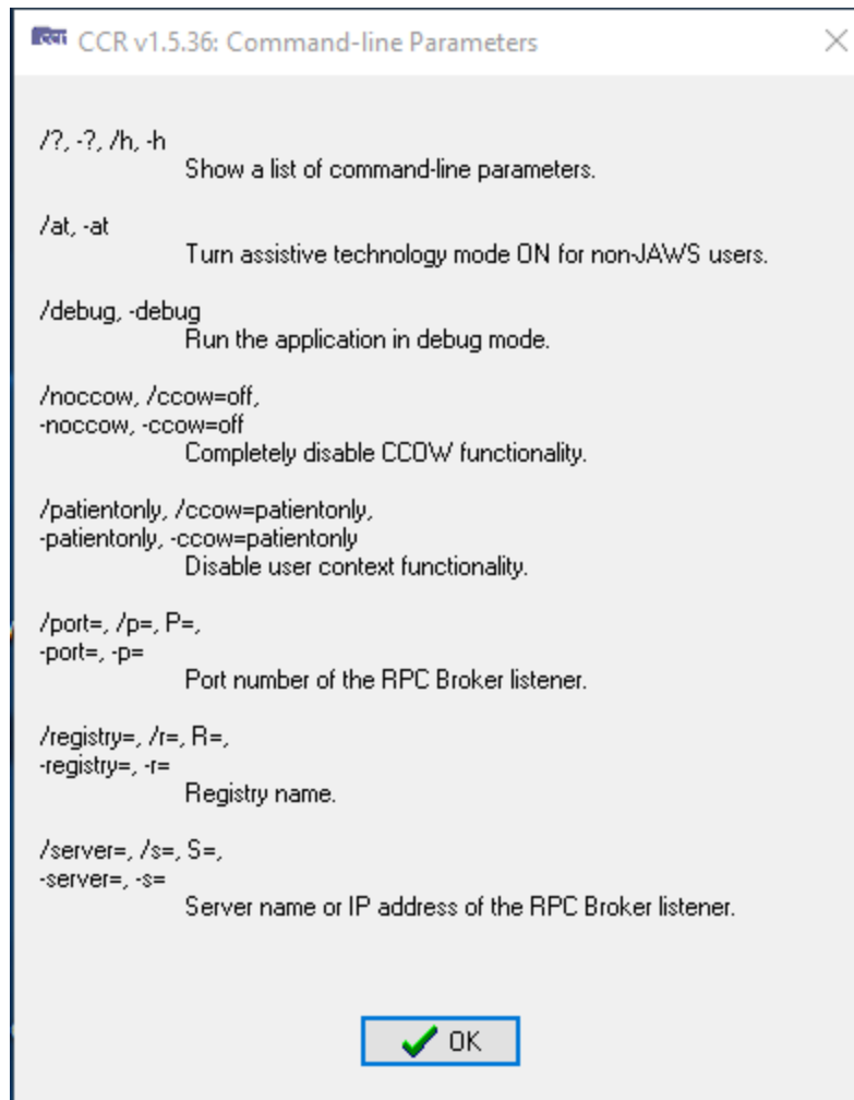
Figure 10 – Command-Line Switches
