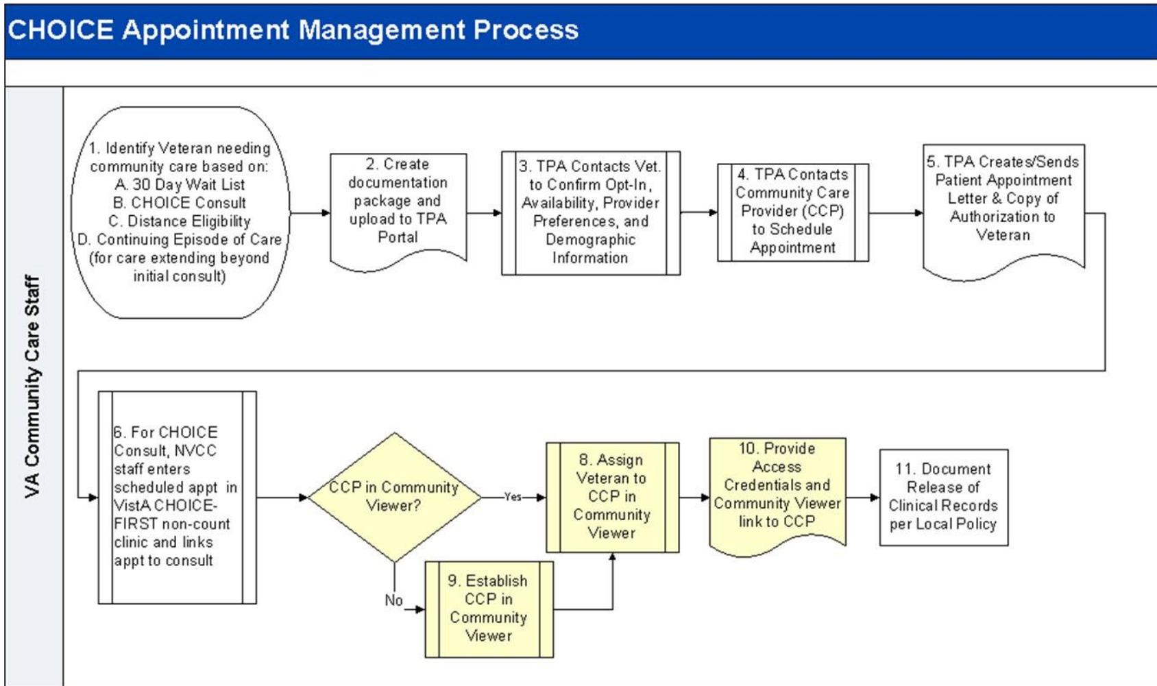
Figure 1: User Workflow
