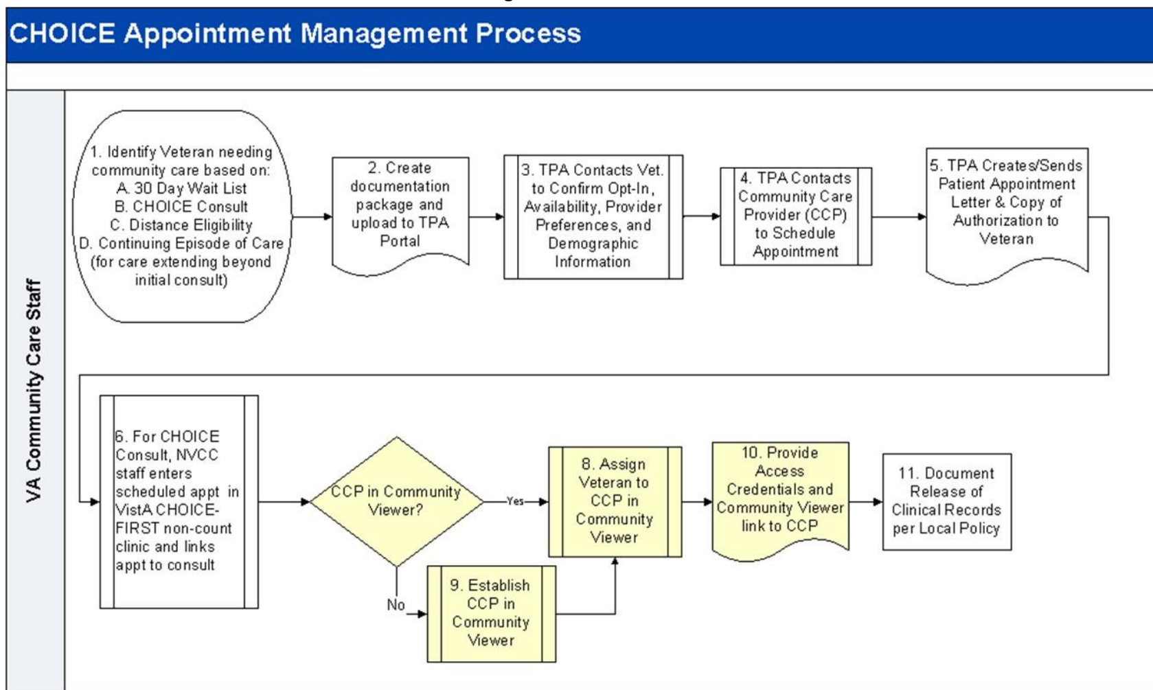
Figure 2: User Workflow
