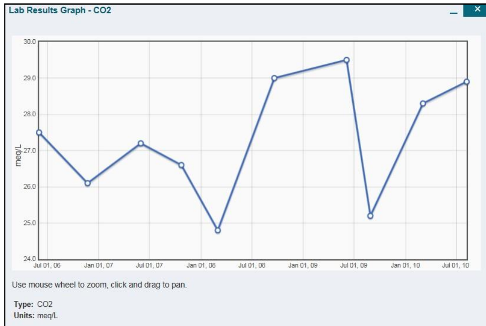
Figure 36: Graph View
