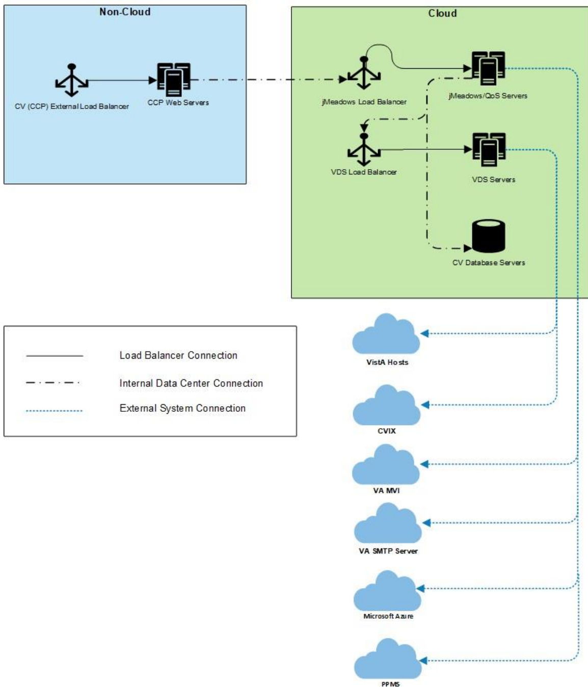
Figure 2: CV CCP Production Architecture Community Viewer – CCP Production
