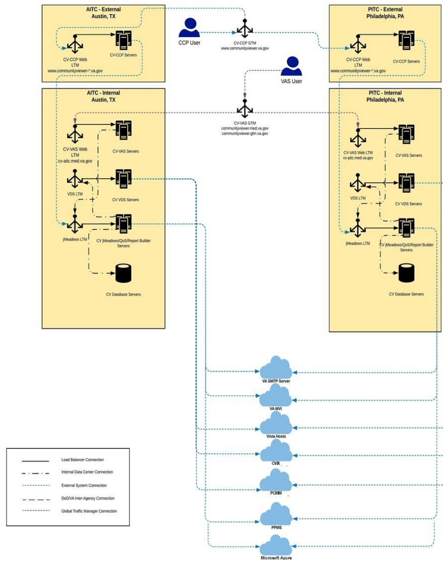
Figure 1: CV Production Hardware Architecture 2
