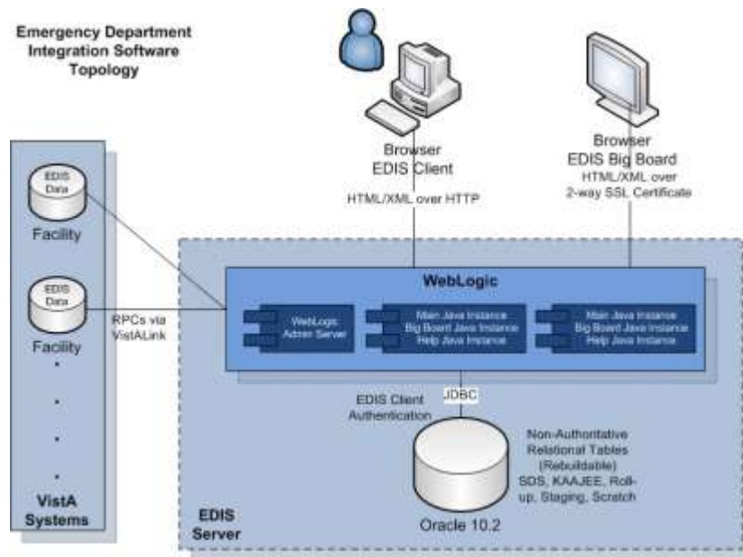
Figure 1: The EDIS Topology
