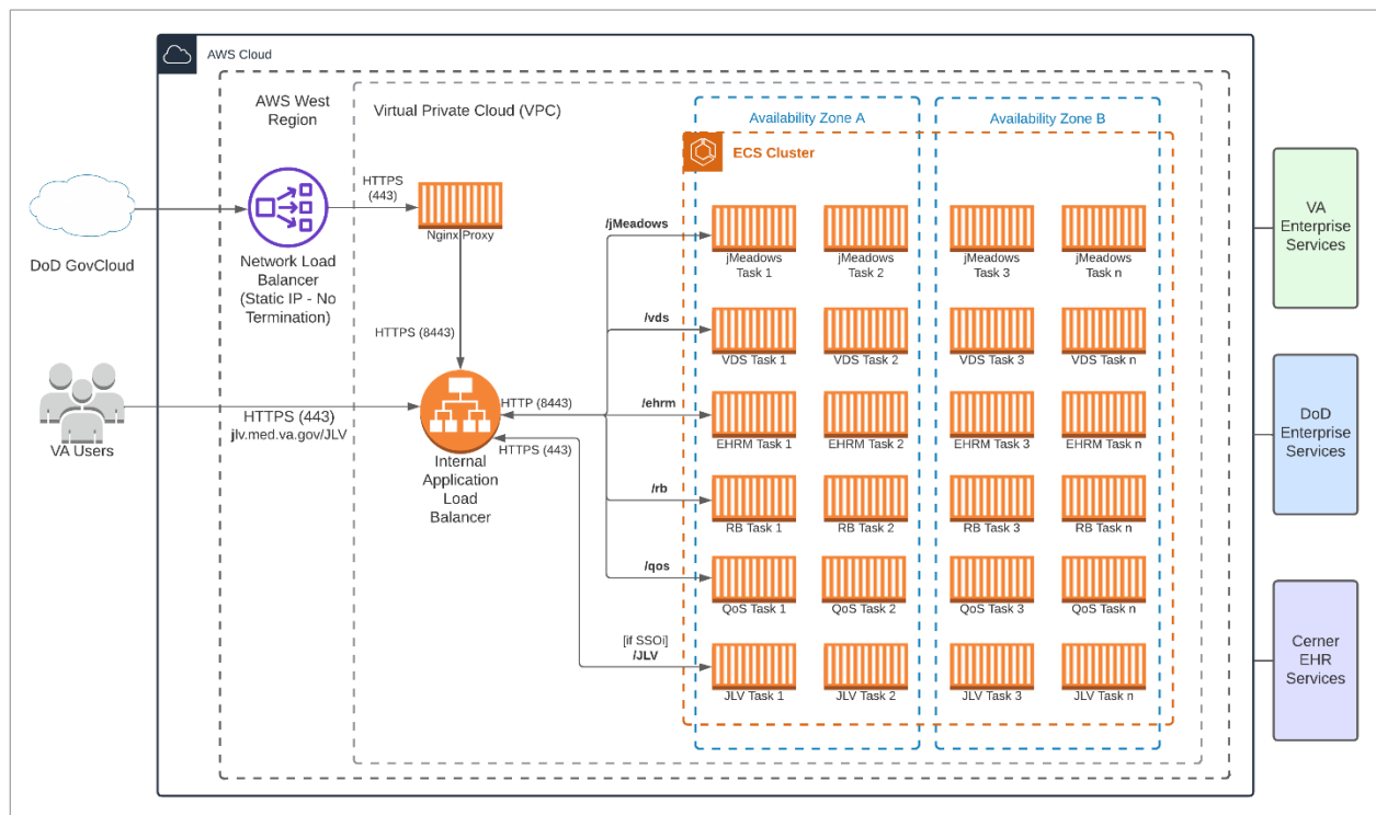
Figure 3: JLV Topology 3
