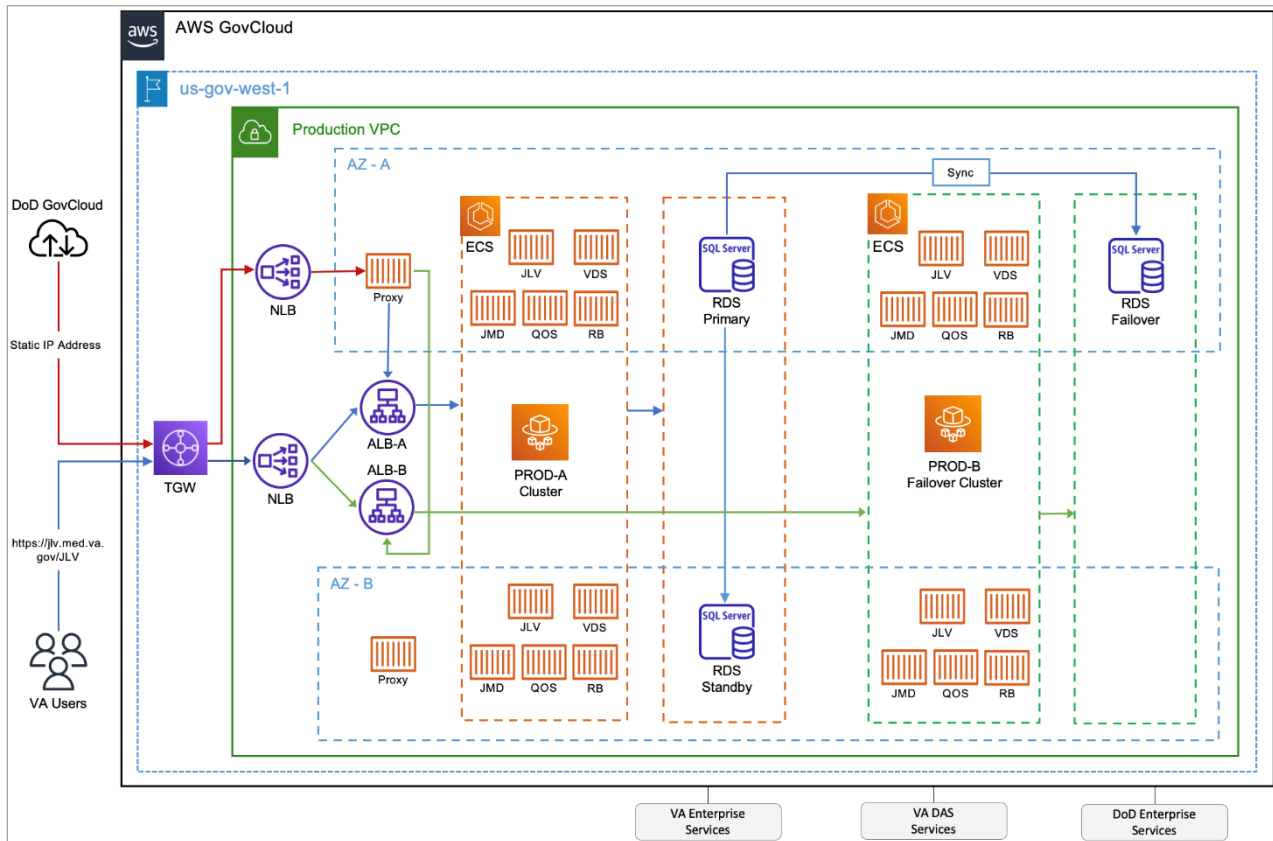
Figure 3: JLV Topology 3
