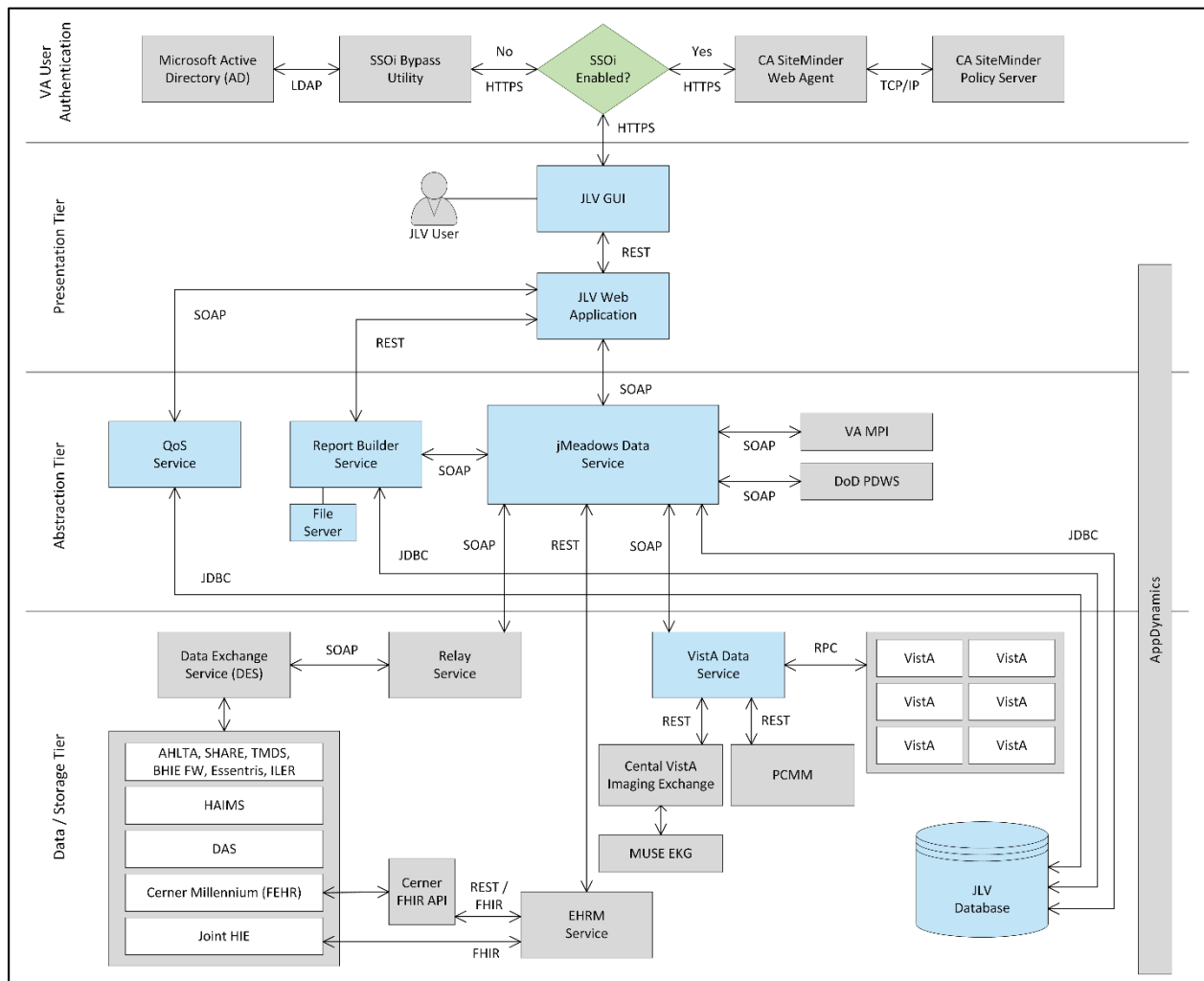
Figure 18: JLV Architecture and Components 5
