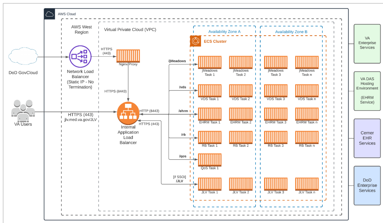
Figure 3: JLV Topology 3
