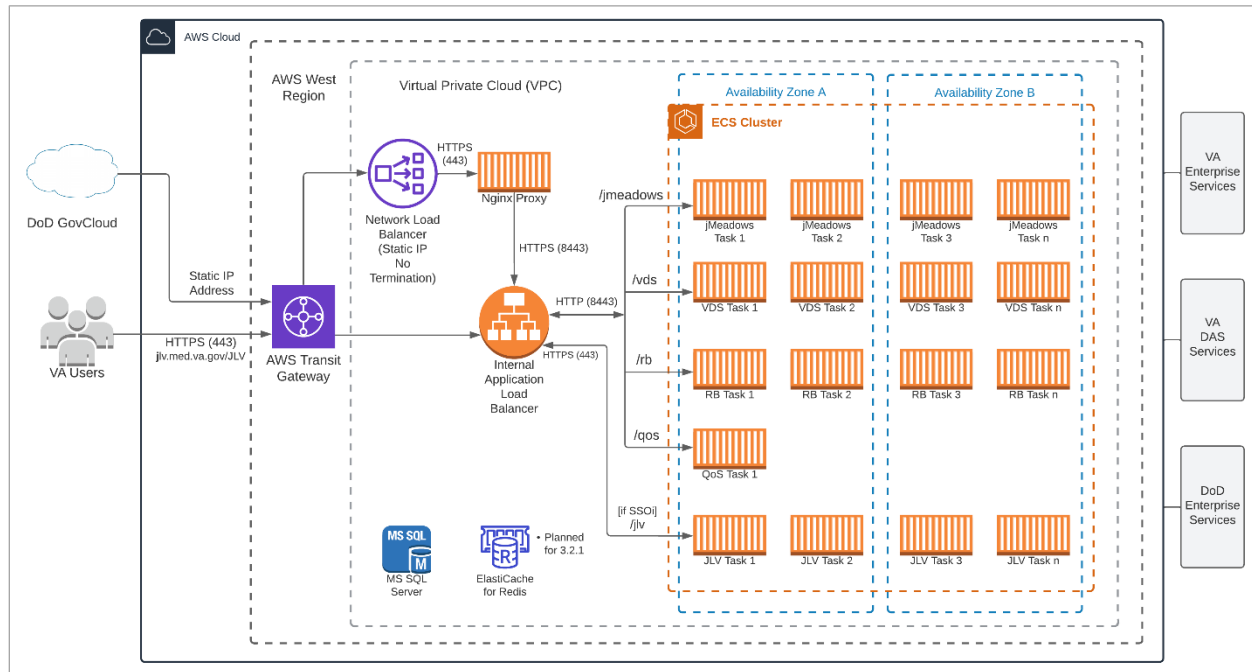
Figure 3: JLV Topology 3
