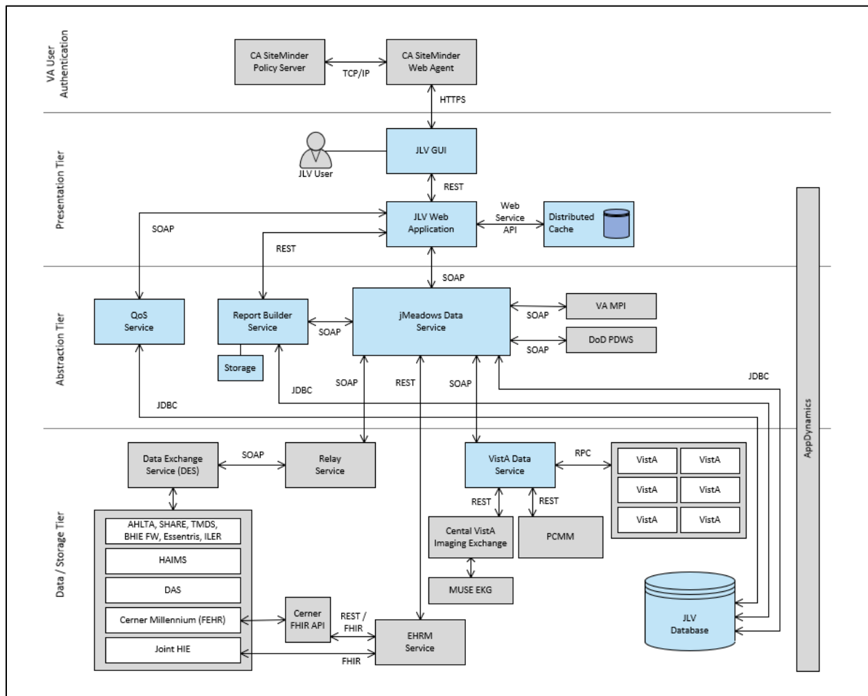
Figure 1: JLV Architecture and Components 2
