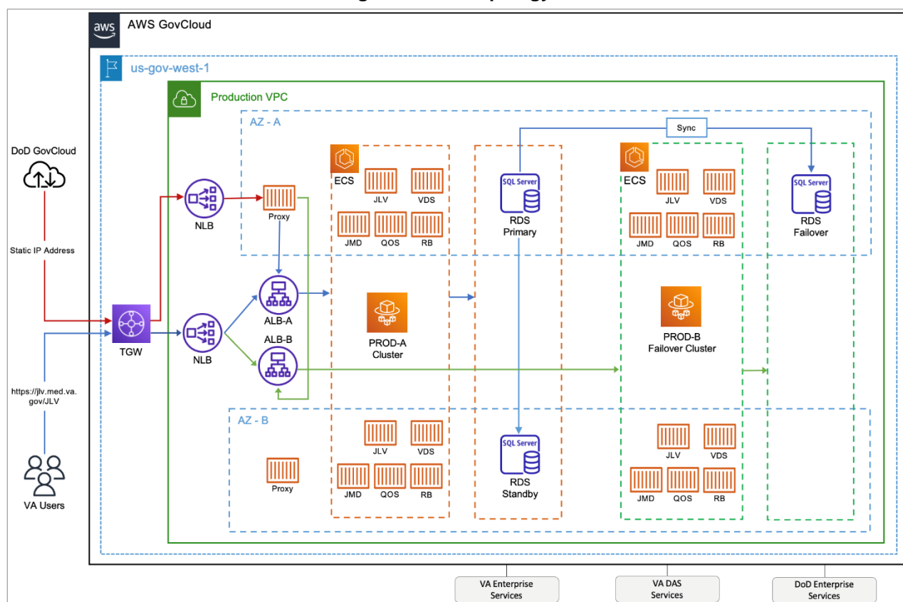
Figure 3: JLV Topology 3
