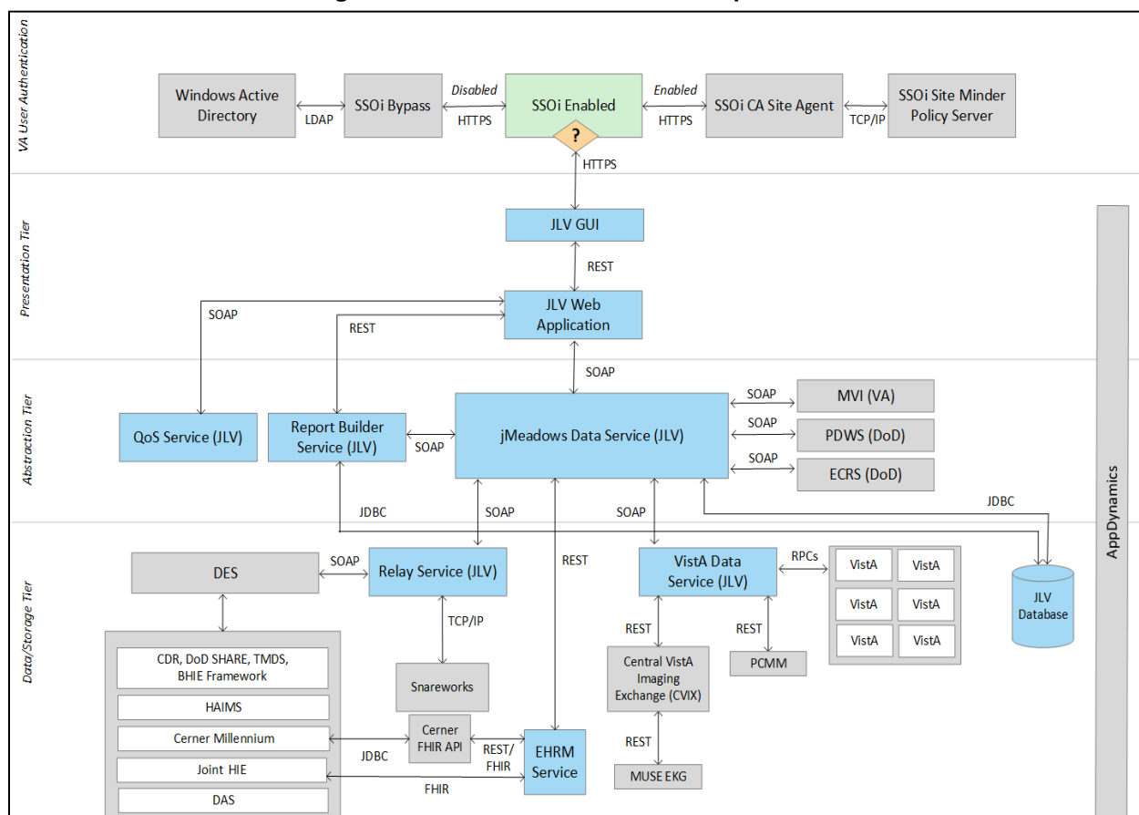
Figure 1: JLV Architecture and Components 2
