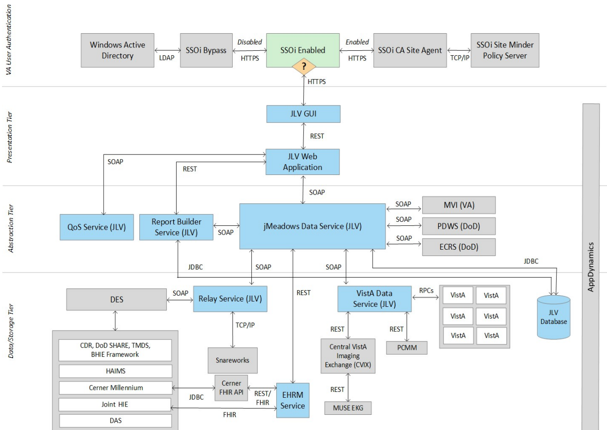
Figure 21: JLV Architecture and Components 4
