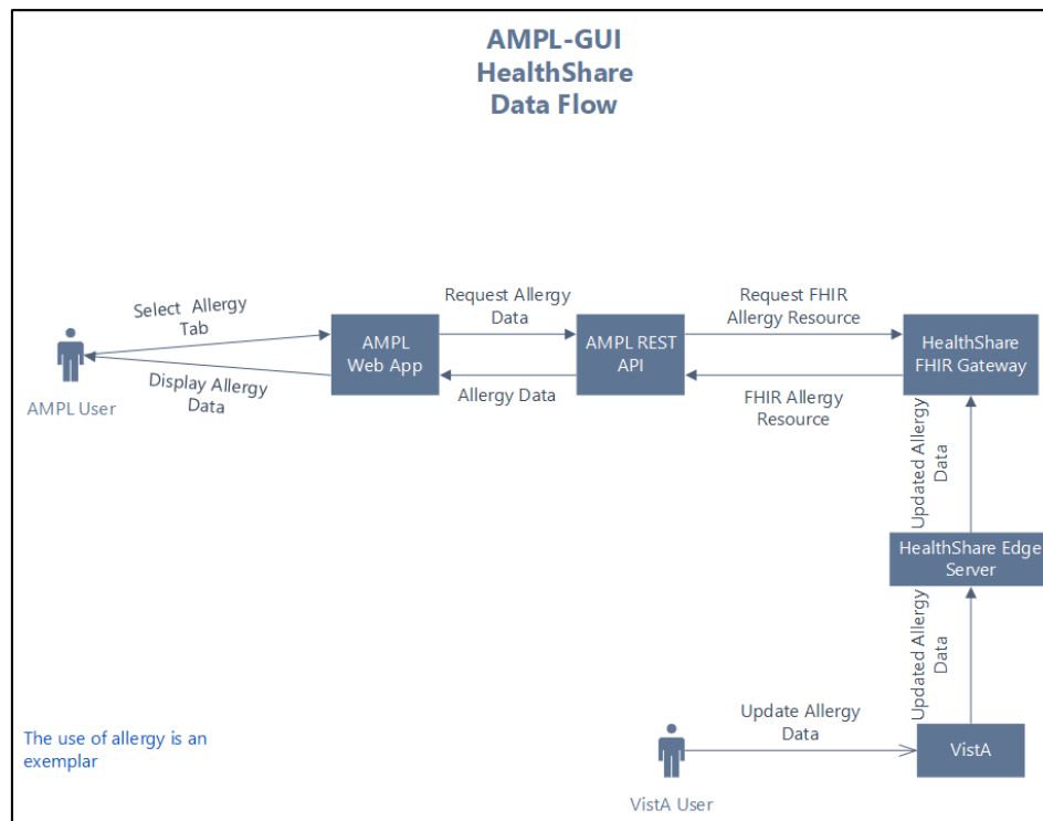
Figure 1: Logical High-Level AMPL GUI HealthShare Data Flow
