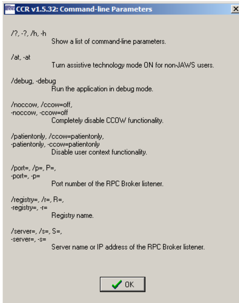
Figure 10 – Command-Line Switches
