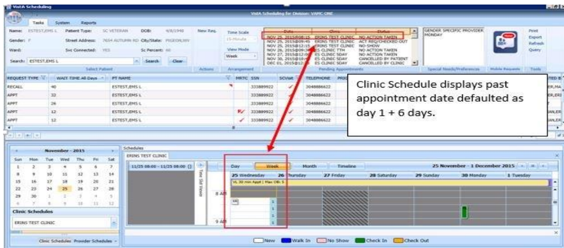
Figure 82: Clinic Schedule Grid – Past Appointment Display
