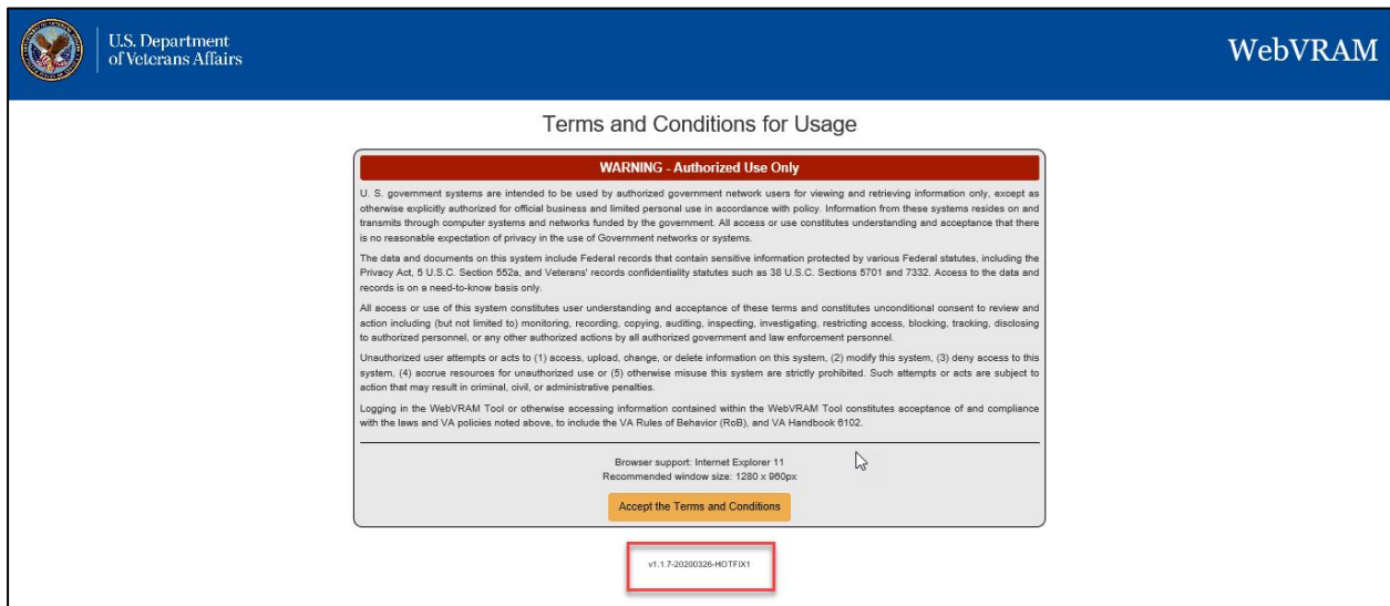
Figure 3: WebVRAM Homepage
