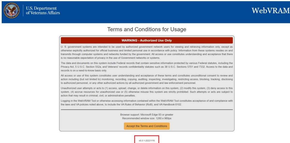
Figure 3: WebVRAM Homepage
