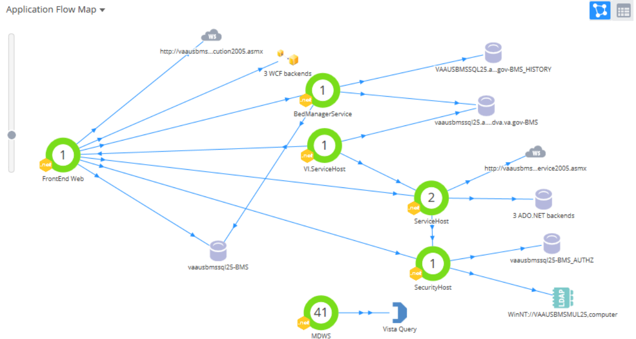
Figure 71- Application Flow map from APPDYNAMICS
