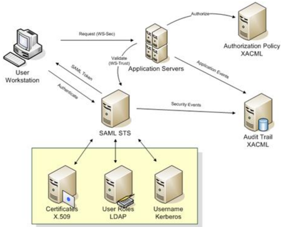
Figure 43- Security Services Architecture
