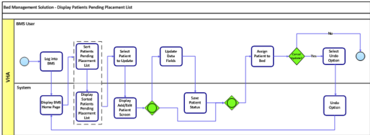
Figure 61- Display and Update PPBP Business Process
