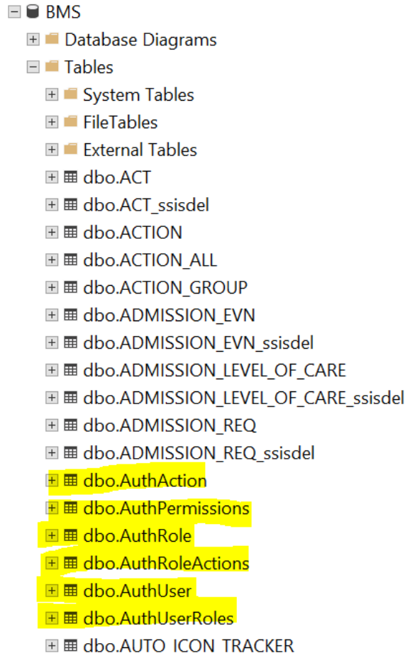
Figure 44- New tables added to BMS database for Policy Manager Replacement
