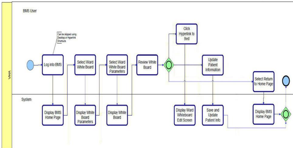
Figure 66- Manage Whiteboard Business Process
