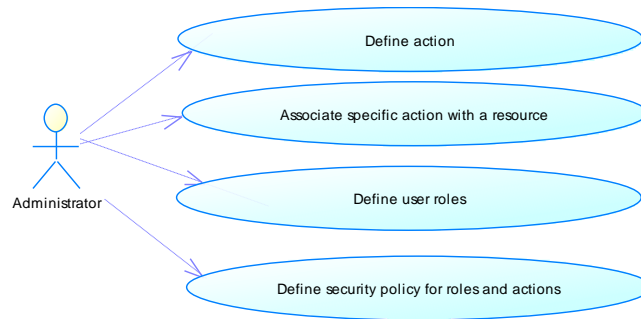
Figure 53- Authorization Administration Use Cases
