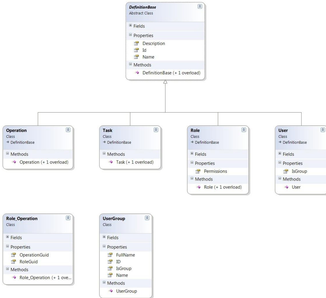
Figure 54- Class Diagram for Data Contracts in PAP and PDP
