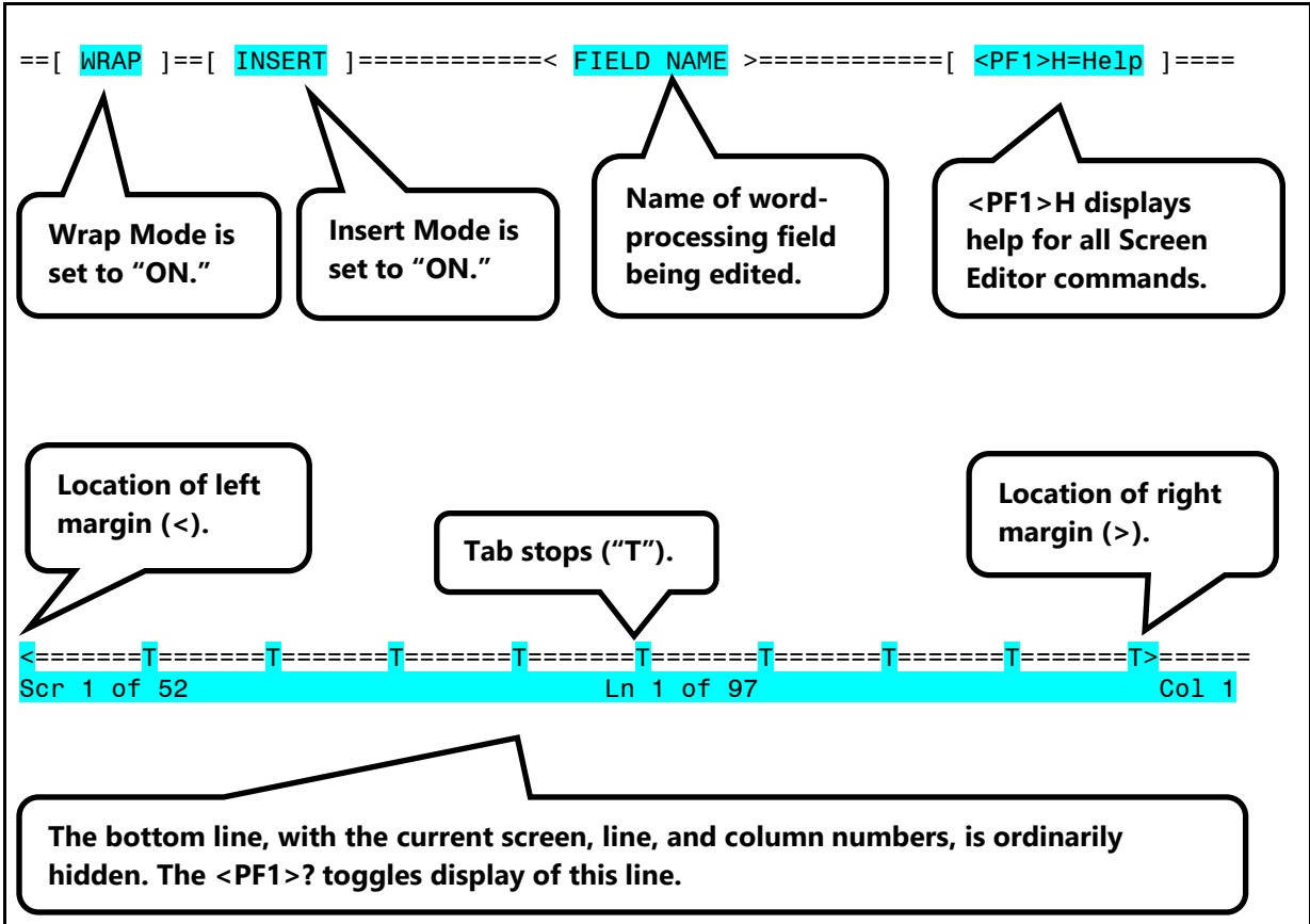
Figure 103: Screen Editor—Sample WORD-PROCESSING Field in the Screen Editor: Sample Component Parts
