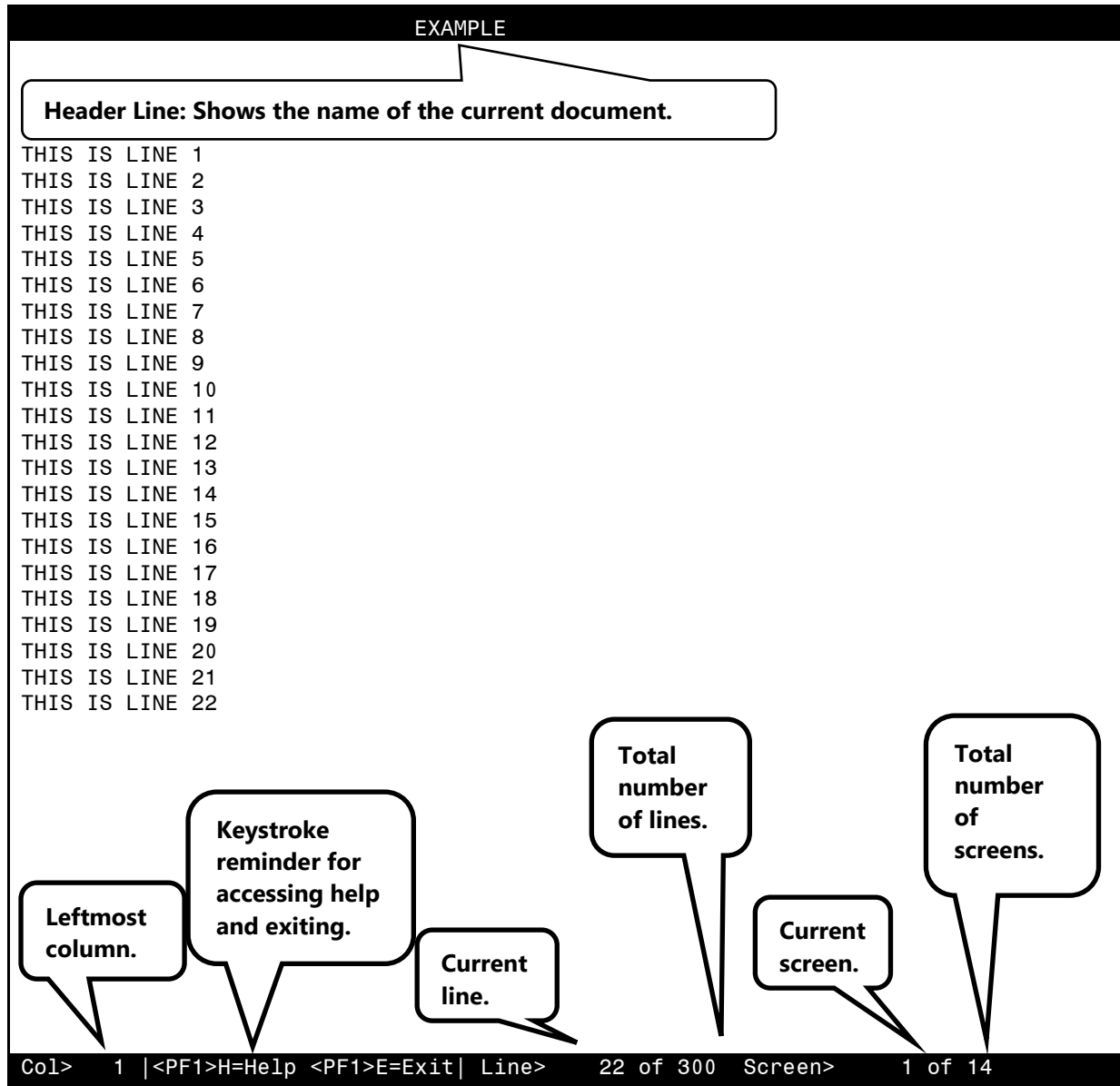
Figure 50: Browser—Sample Screen Component Parts
