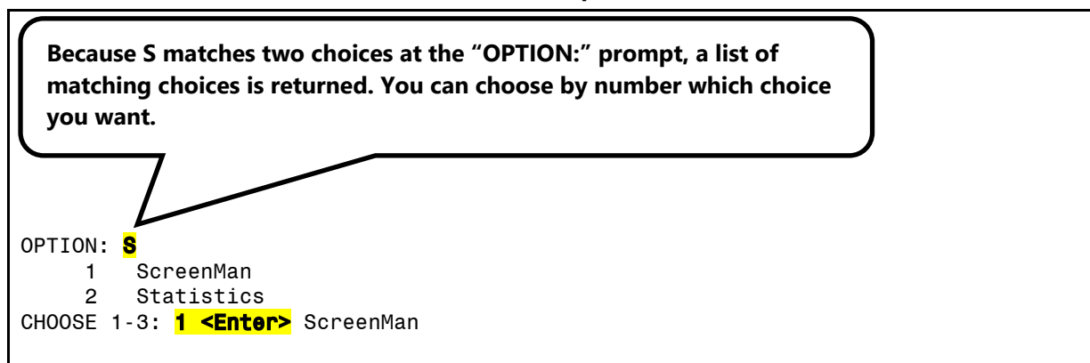
Figure 55: VA FileMan Prompts—Dialog to Choose from a List in VA FileMan: Sample User Entries at Prompts
