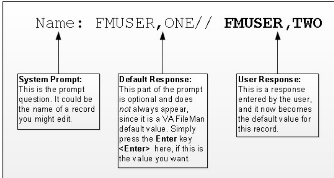
Figure 51: VA FileMan Prompts—Sample Component Parts of a Prompt
