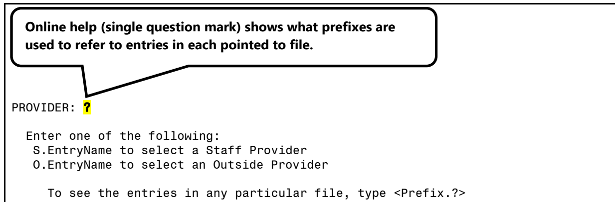
Figure 81: Field Types—Dialog Showing Help for Entries in a VARIABLE-POINTER Field: Sample User Entries at Prompts
