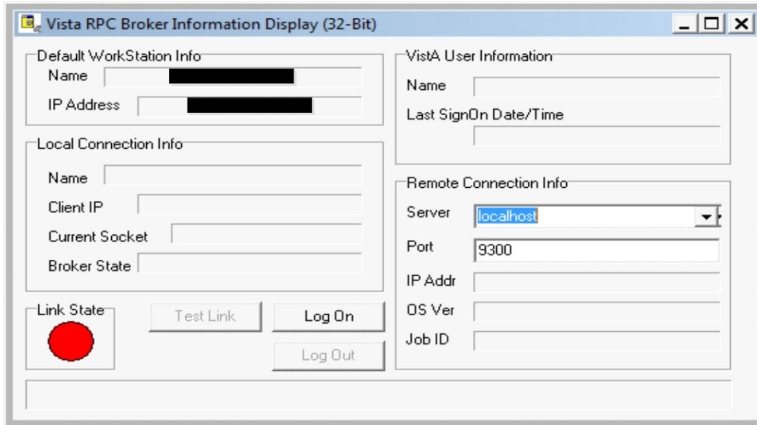
Figure 3: RPC Broker Connection Diagnostic Application
