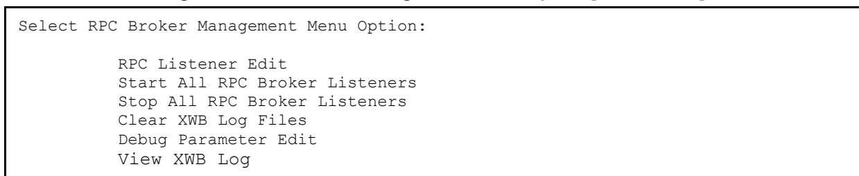
Figure 2: RPC Broker Management Menu Option [XWB MENU]
