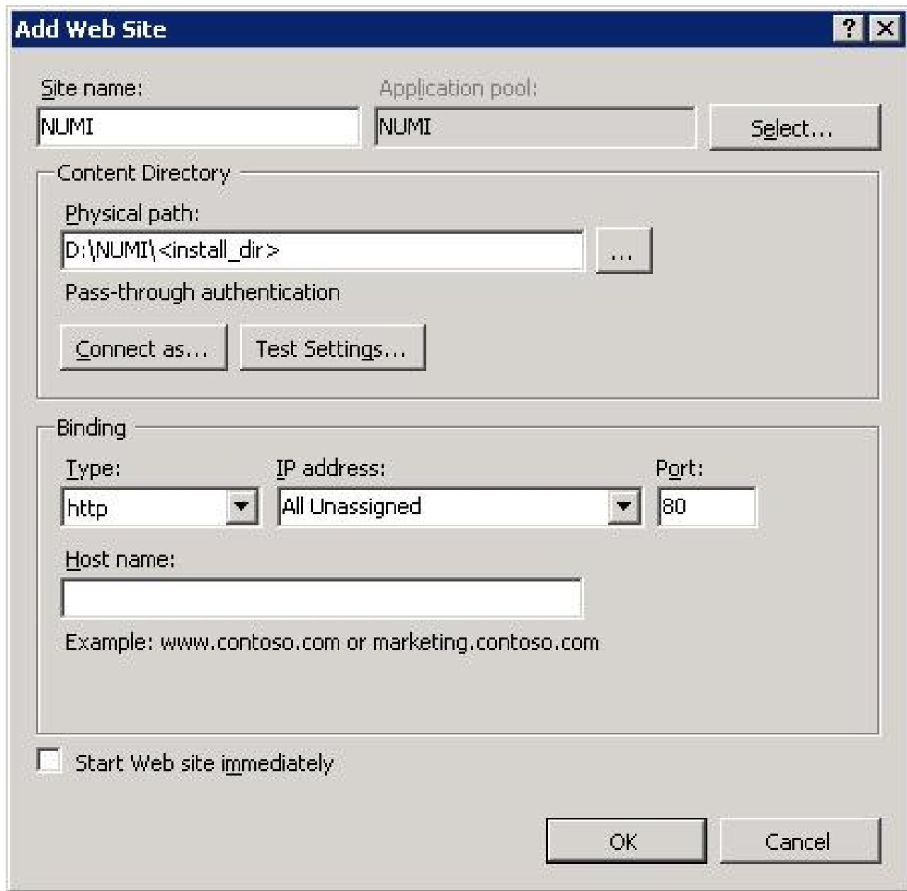
Figure 32: Add NUMI Website
