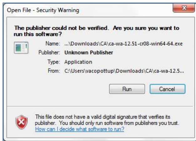
Figure 42: Security Warning
