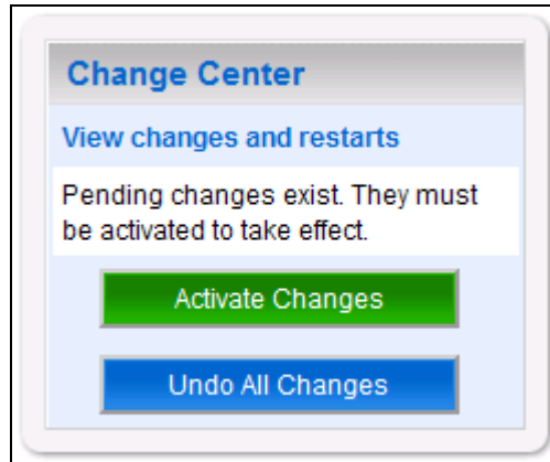
Figure 3-90. Activate Changes
