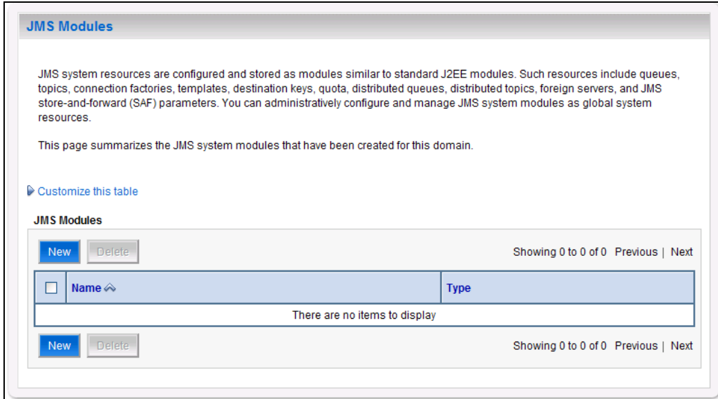
Figure 3-36. JMS Modules
