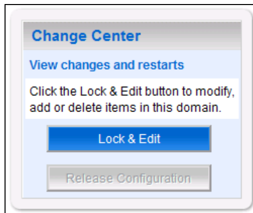
Figure 3-41. Lock & Edit
