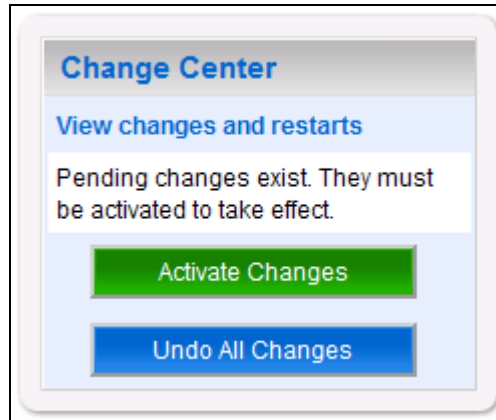
Figure 3-27. Activate Changes
