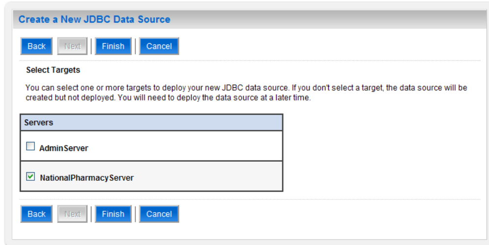
Figure 3-25. Select Targets
