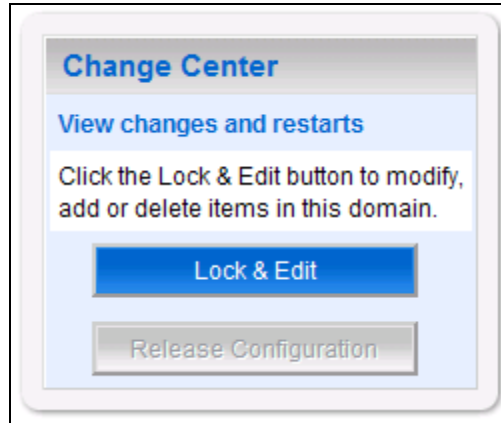
Figure 3-3. Change Center
