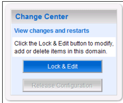
Figure 3-52. Lock & Edit
