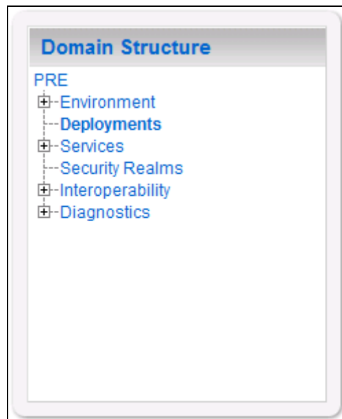
Figure 3-91. Domain Structure
