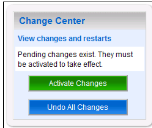
Figure 3-7. Activate Changes
