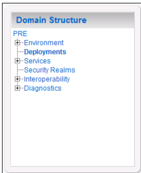
Figure 3-79. Domain Structure
