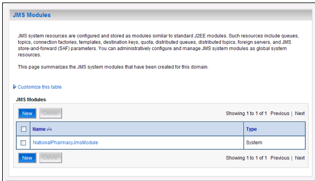
Figure 3-64. JMS Modules
