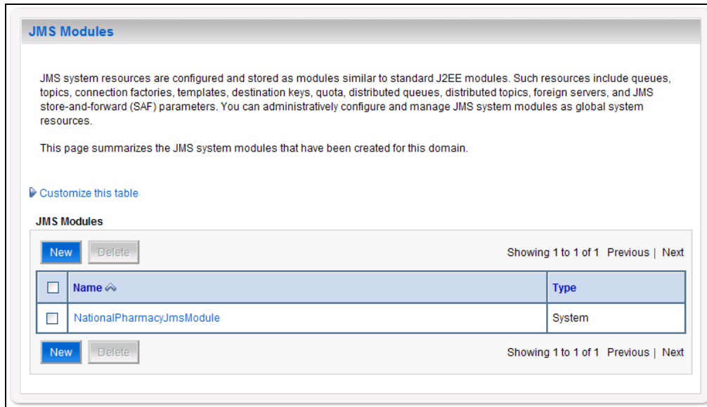
Figure 3-54. JMS Modules
