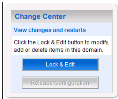
Figure 3-62. Lock & Edit
