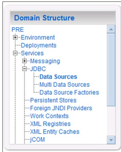
Figure 3-8. Domain Structure
