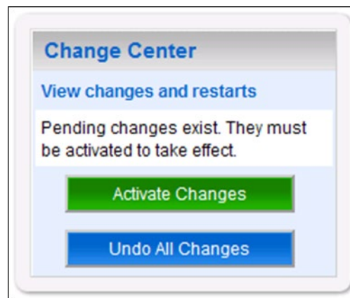
Figure 3-18. Activate Changes
