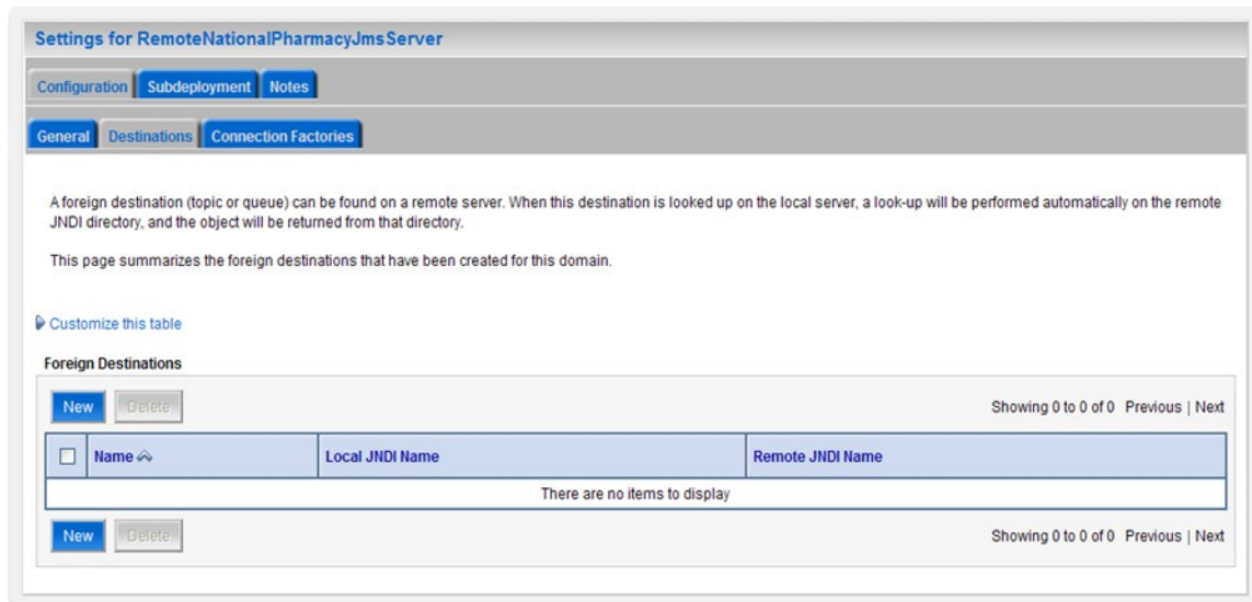
Figure 3-41. Destinations
