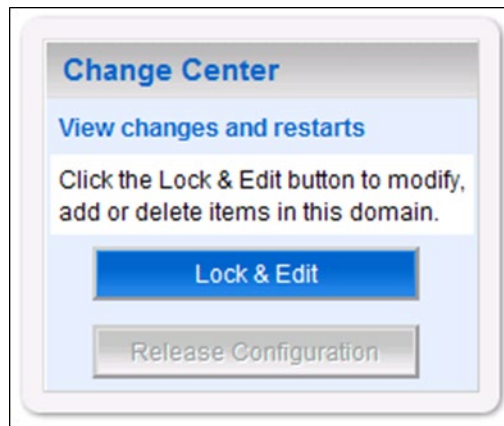
Figure 3-53. Change Center
