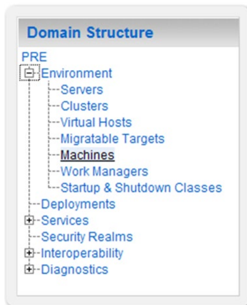
Figure 3-2. Domain Structure
