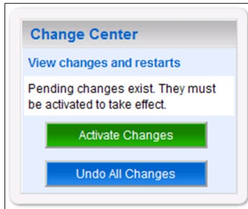
Figure 3-63. Activate Changes
