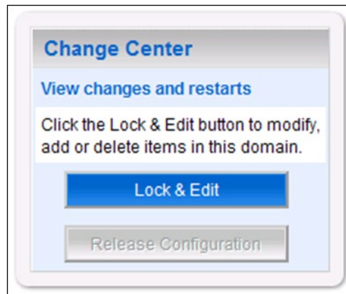
Figure 3-3. Change Center
