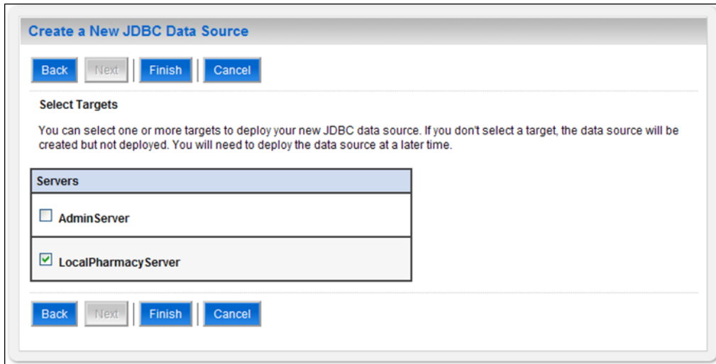
Figure 3-15. Select Targets
