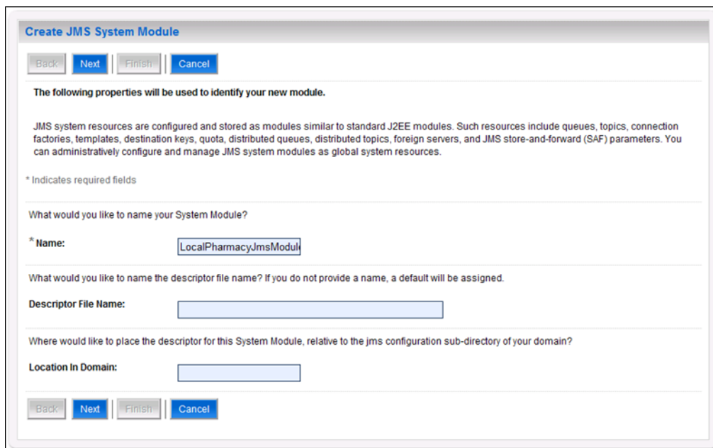
Figure 3-22. JMS System Module Properties
