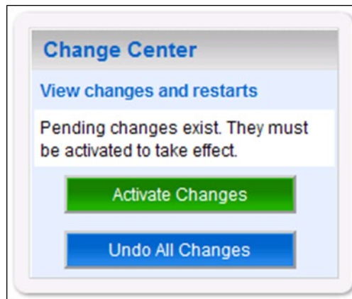
Figure 3-35. Activate Changes
