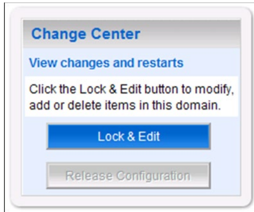
Figure 3-44. Lock & Edit
