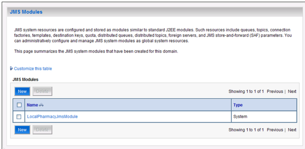
Figure 3-28. JMS Modules
