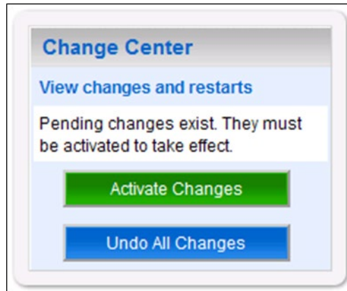
Figure 3-25. Activate Changes
