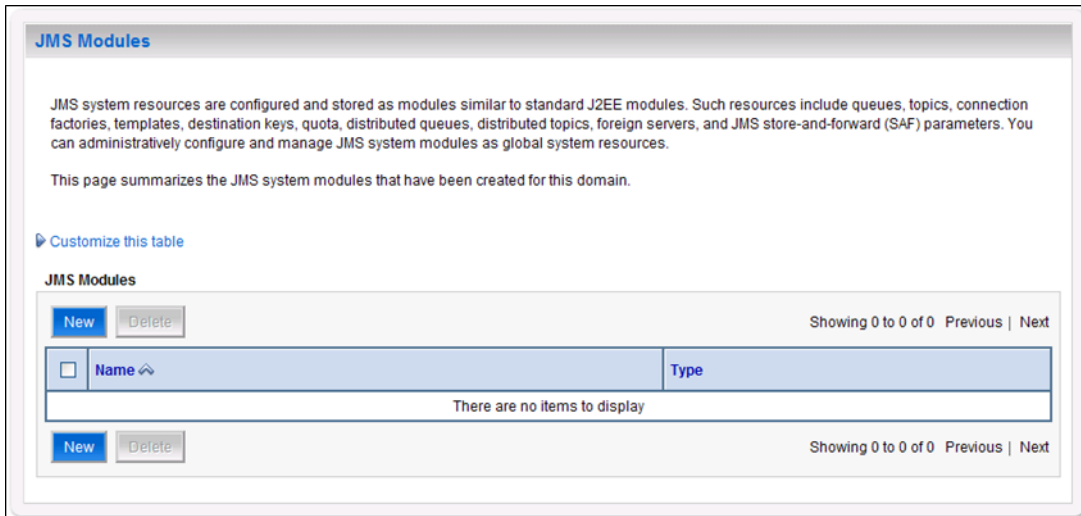
Figure 3-21. JMS Modules
