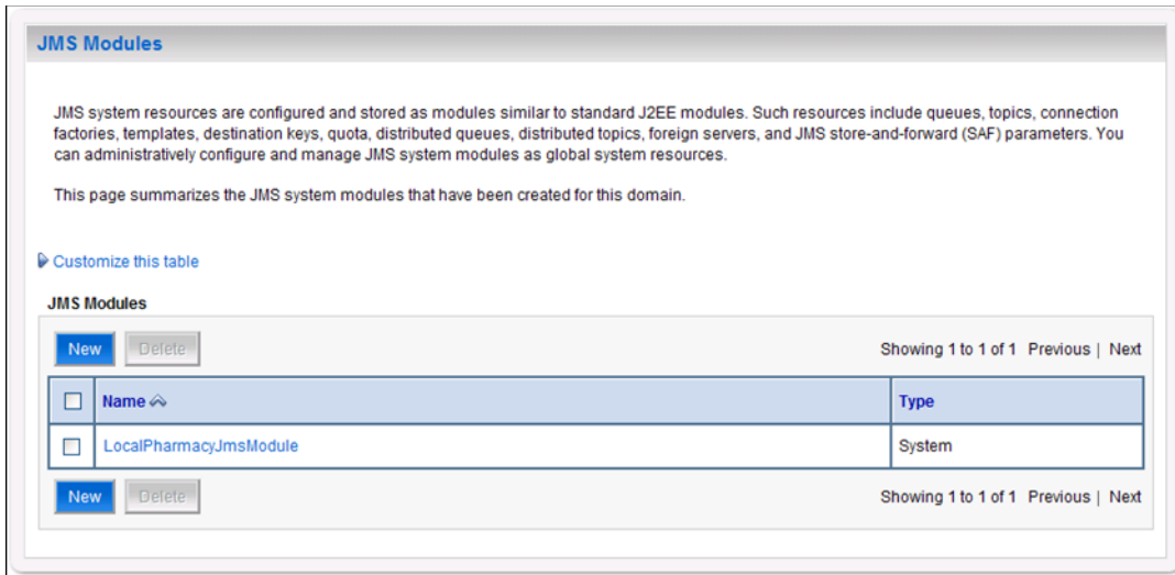
Figure 3-46. JMS Modules
