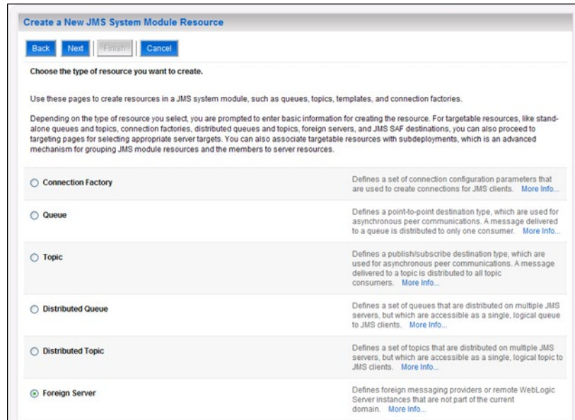
Figure 3-30. Choose Type of Resource to Create
