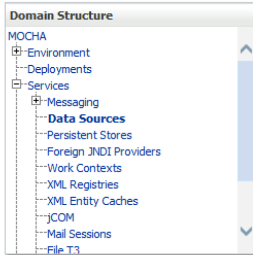
Figure 3-8. Domain Structure
