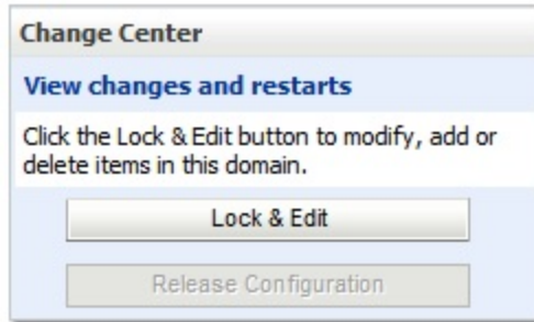
Figure 3-28. Change Center
