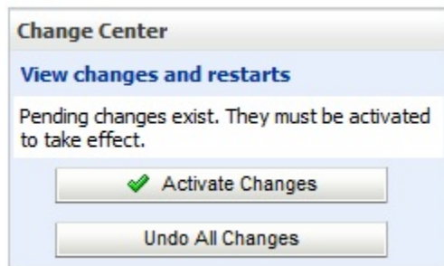
Figure 3-37. Activate Changes
