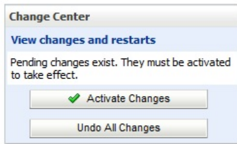
Figure 3-26. Activate Changes
