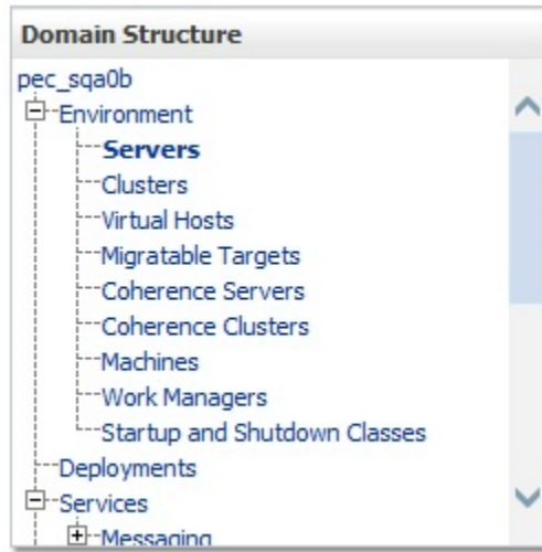
Figure 3-38. Domain Structure
