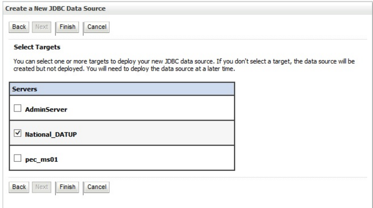
Figure 3-24. Select Targets
