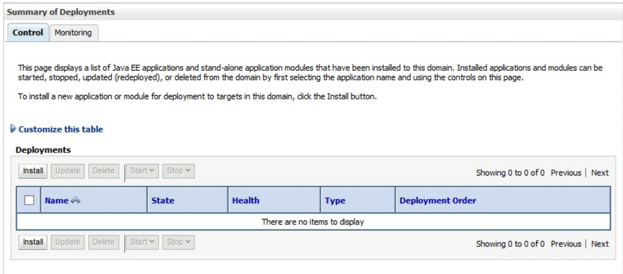
Figure 3-29. Deployments
