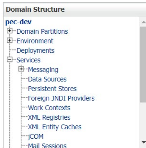
Figure 42: Domain Structure
