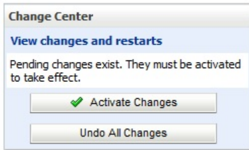
Figure 26. Activate Changes
