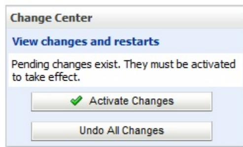
Figure 37: Activate Changes
