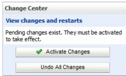
Figure 49: Activate Changes
