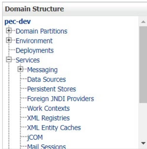
Figure 38: Domain Structure
