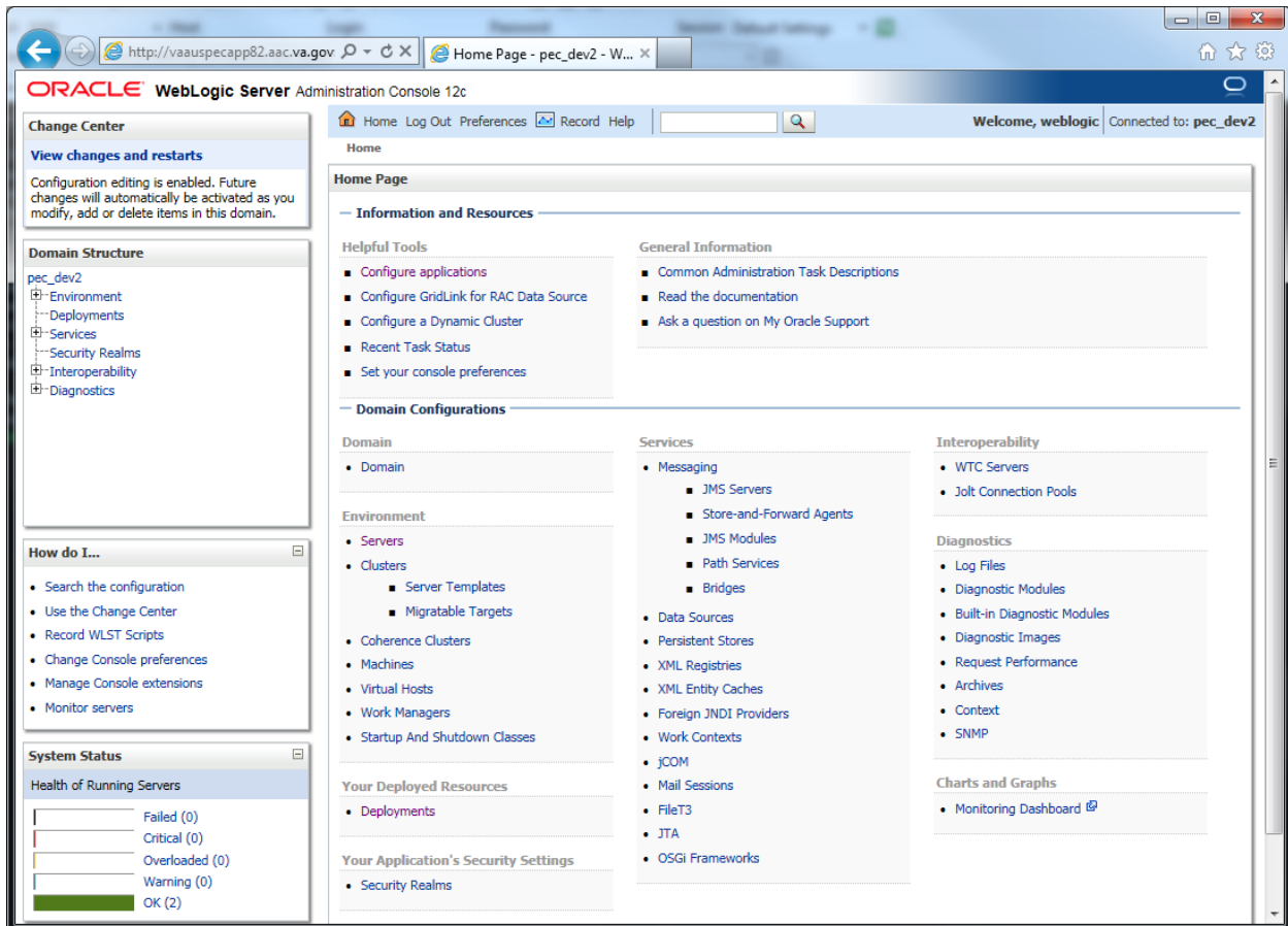
Figure 1: WebLogic Console
