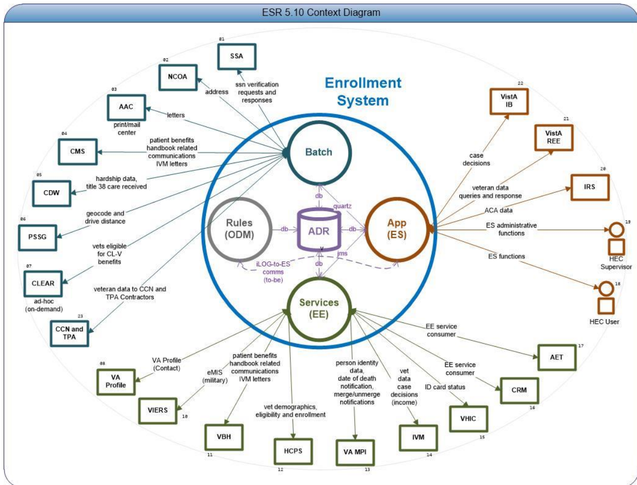
Figure 1: Dataflow Diagram
